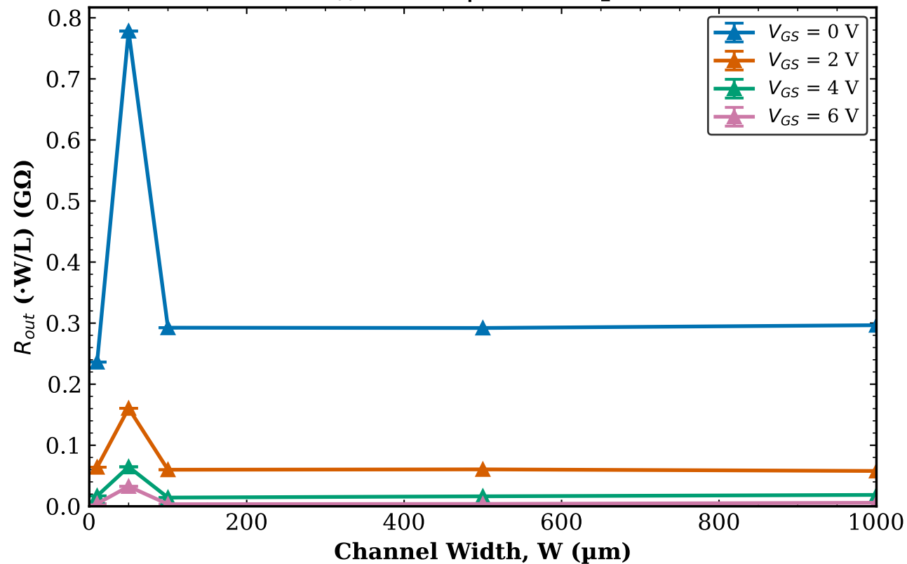
TFT1 Transistor 1 R_{out} vs W | L = 10\text{ }\mu\text{m}
